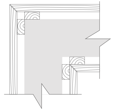
Cut the boards to a 45-degree angle.
