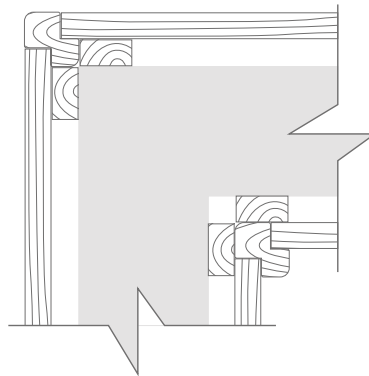
Corner profile CP3
